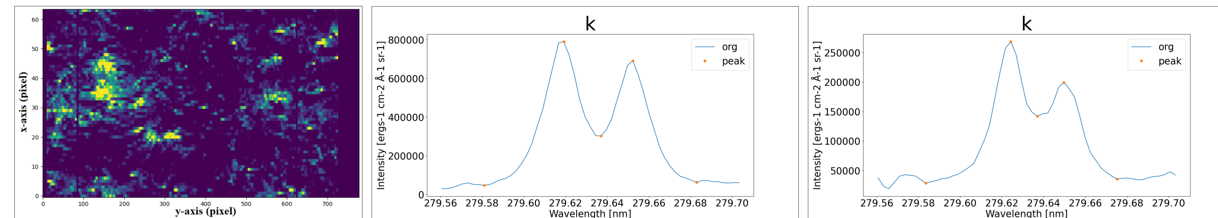
Figure 2: Mg II k spectra for two different pixel locations showing the variation of intensity in the raster taken on July 23, 2019. The left image represents a spectroheliogram in k line (in pixel). The middle image describes a bright region at pixel location [30, 40], while the right image describe a darker region at pixel location [10, 380]. The five orange points on the line profiles show the positions of the spectral features of interest automatically obtained by our algorithm.
