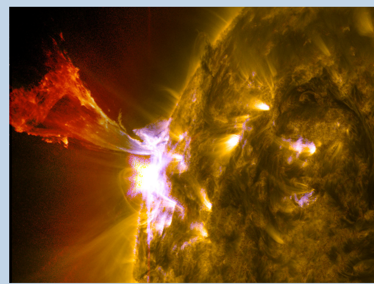
Figure 1: Burst of solar material leaps off the left side of the Sun in what's known as prominence eruption (Credit: NASA/SDO/AIA)
