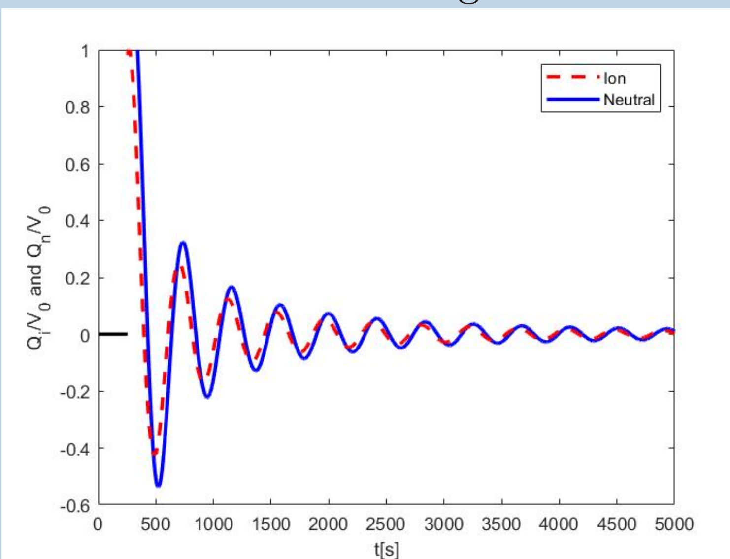
Figure 3: The temporal evolution of neutral-acoustic (solid lines) and ion-acoustic (dashed lines) modes at z = 4 Mm (Alharbi et al. MNRAS, 2021.)
