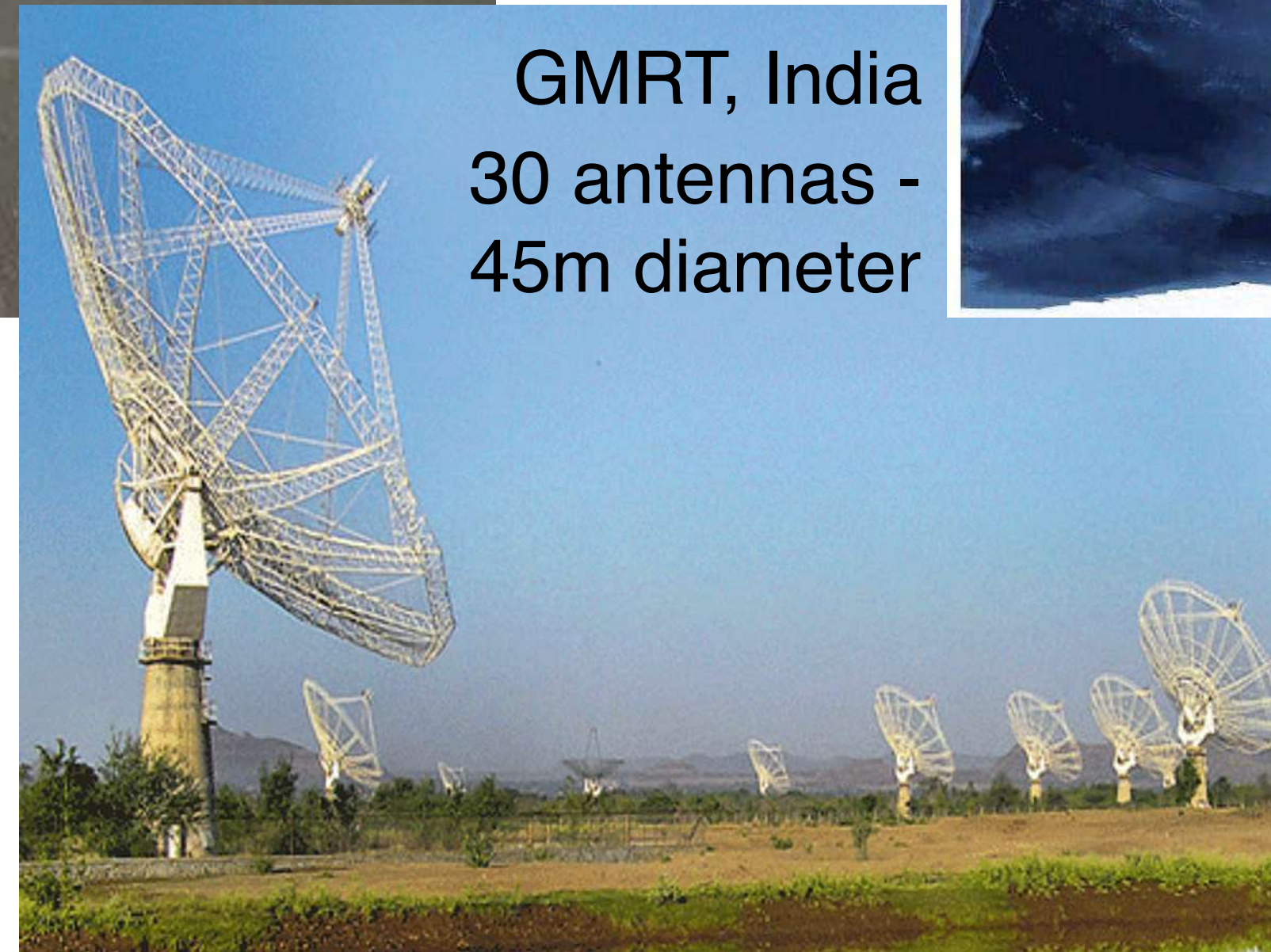
Arcsec resolution
