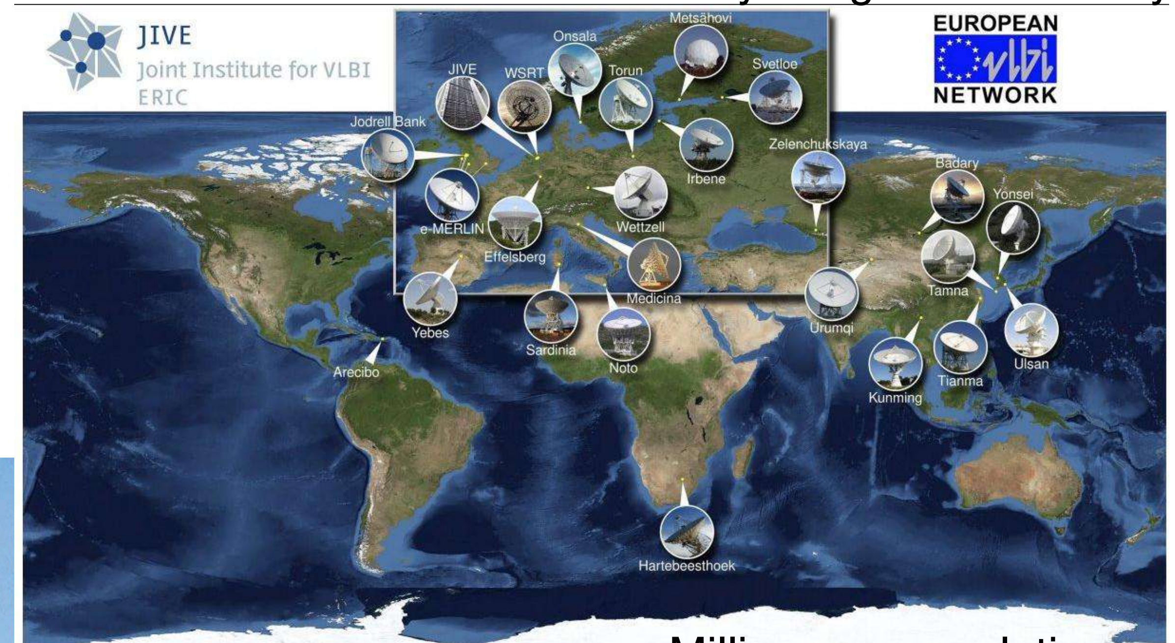
Milli-arcsec resolution
