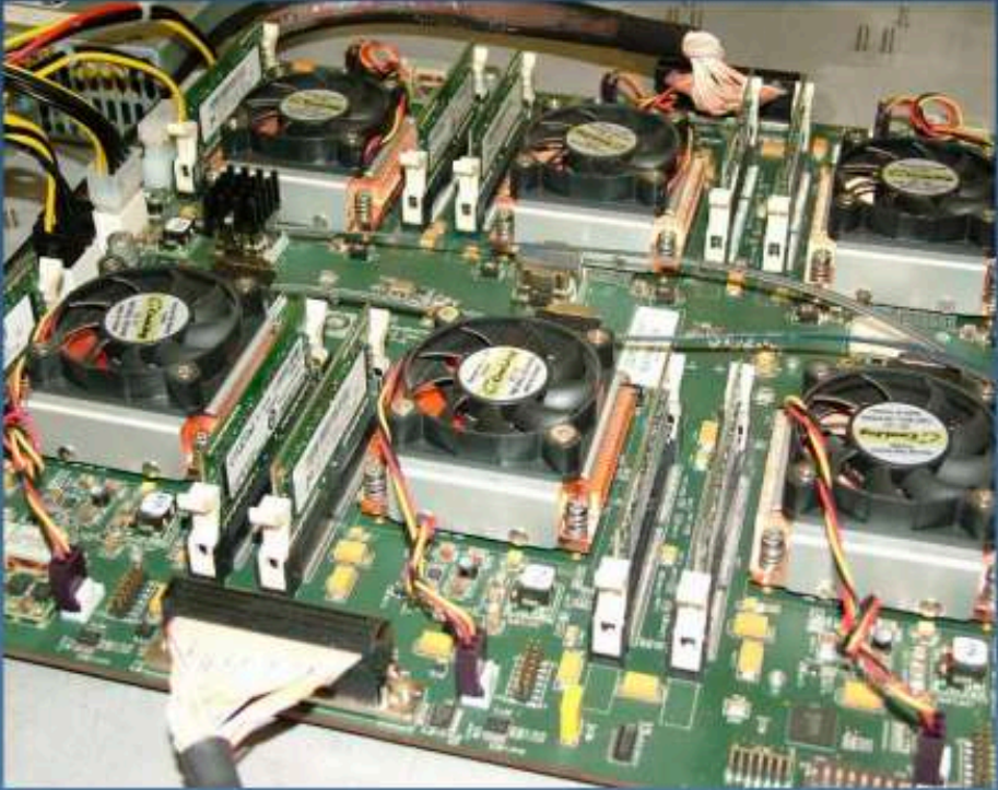
e.g. FPGAs in the ASKAP correlator
