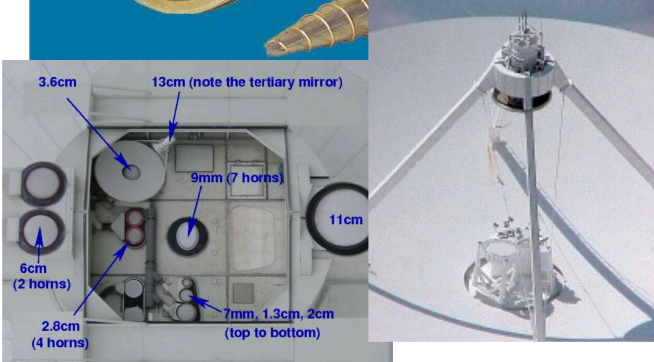
Effelsberg secondary focus
