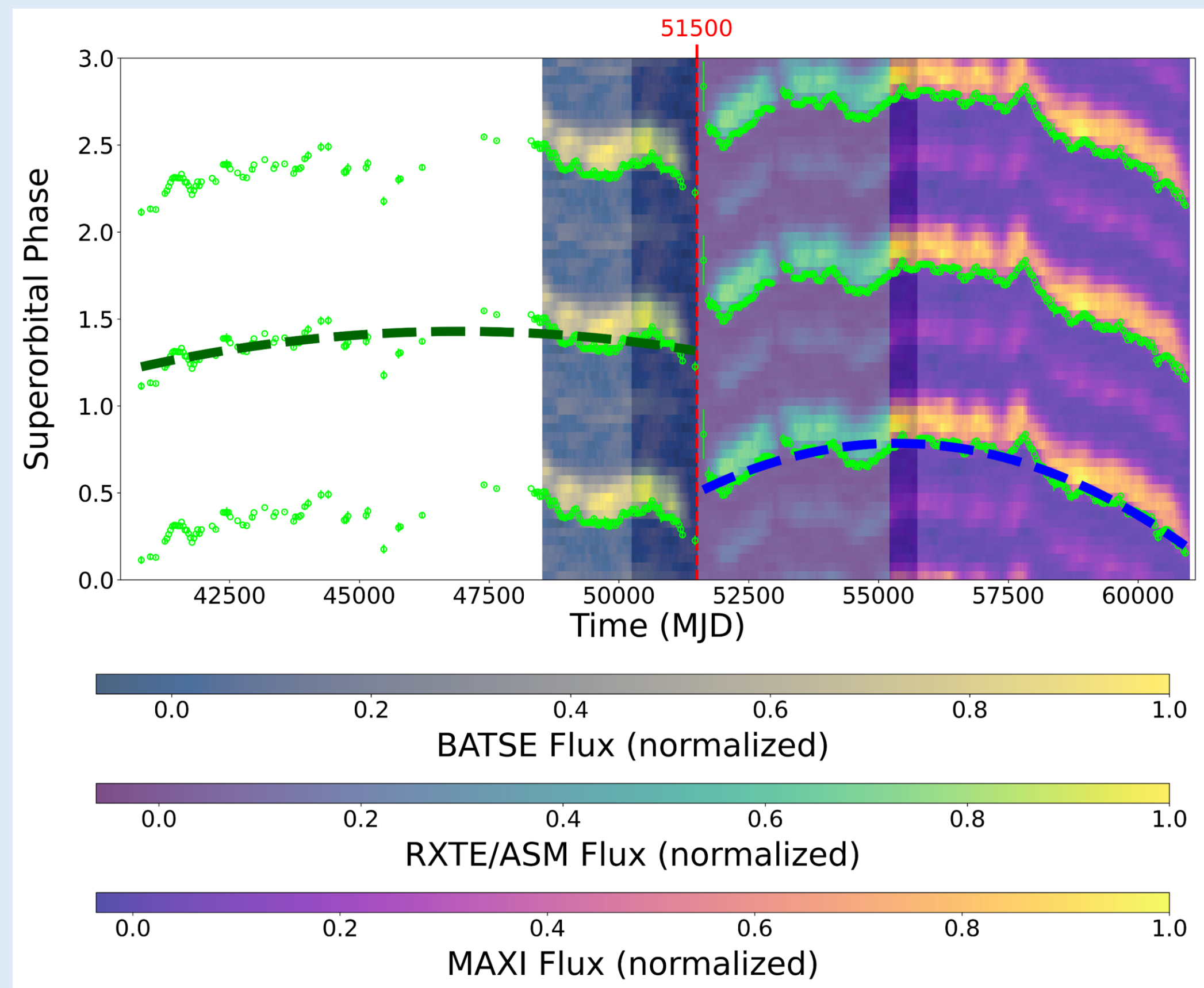
Fig. 3: O–C diagram for Her X-1 ( P_{pr} = 34.85d ; T_0 = 55000 MJD). The «colored» part of the plot corresponds to data from the X-ray monitors: CGRO/BATSE, RXTE/ASM, and MAXI. The «green points» in the plot correspond to the main Turn-on epochs of the X-ray source, as determined from archival observations. Two epochs of the secular change in the accretion-disk precession period are distinguished (separated by the line T = 51500 MJD; red vertical dashed line), with the rate of period change indicated by the green dashed line, \dot{P}_{pr,1} = 1.4 \times 10^{-5} \text{ s s}^{-1} , and by the blue dashed line, \dot{P}_{pr,2} = 4.7 \times 10^{-5} \text{ s s}^{-1} .
