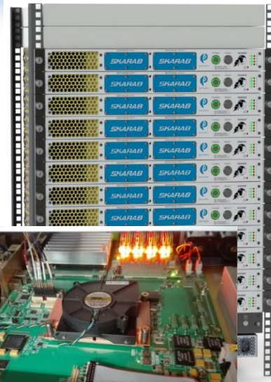
SKARAB ( Square Kilometer Array Reconfigurable Application Board )
