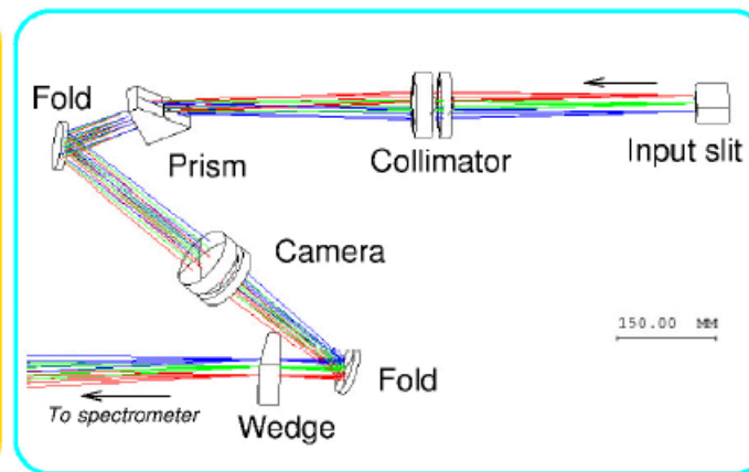
Slit re-imager and anamorphic pupil expander
