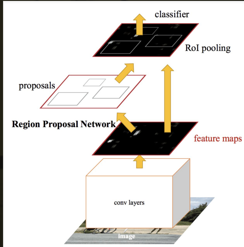
FASTER R-CNN
